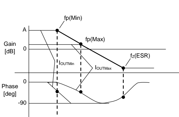
Figure 31. Open Loop Gain Characteristics
