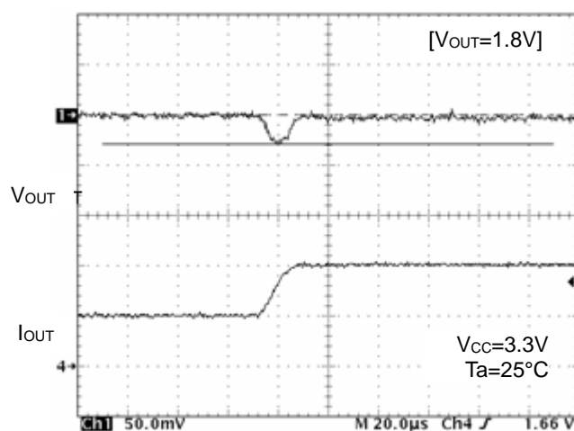
Figure 17. Transient Response ( I_o=1\text{A to }2\text{A}, 10\mu\text{s} )
