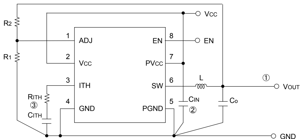
Fig.35 Layout diagram
