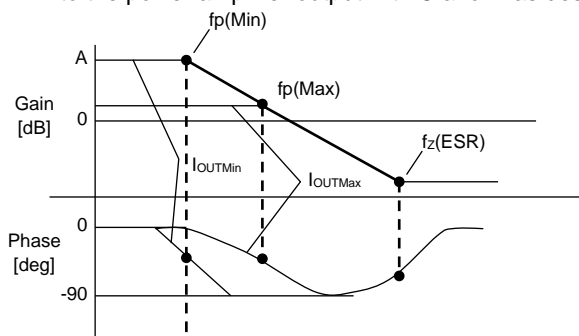
Figure 37. Open Loop Gain Characteristics
