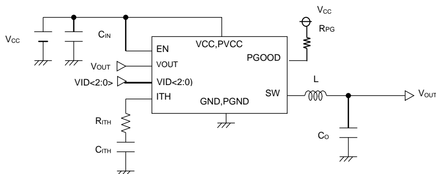
Figure 39. Typical Application
