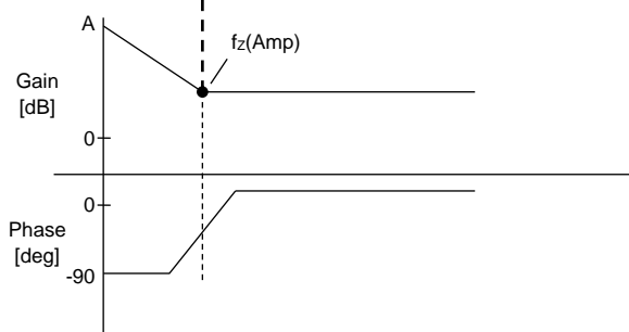
Figure 38. Error Amp Phase Compensation Characteristics
