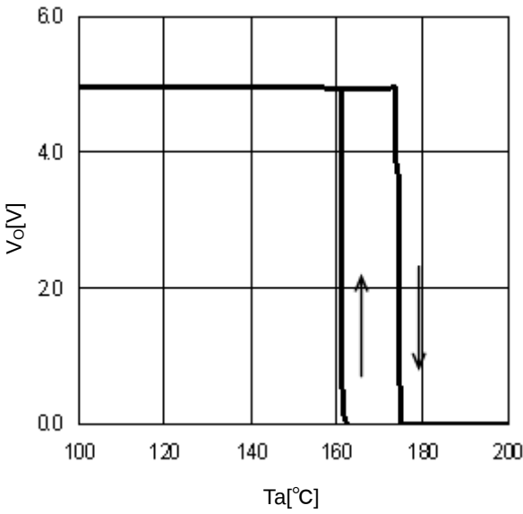
Figure 16. TSD ( I_o=0mA )
