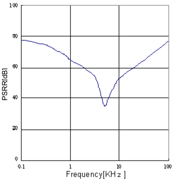
Figure 32. PSRR( I_o=0mA )
