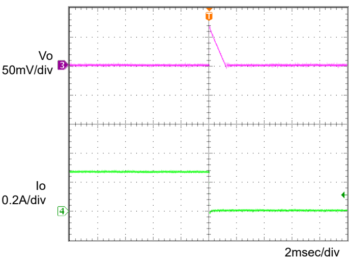
Figure 8. Transient Response (0.3→0A) Co=1μF, Ta=105°C
