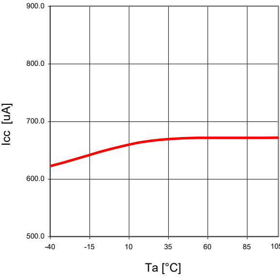
Figure 22. T_a - I_{CC}
