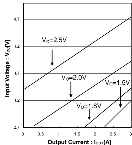
Figure 33. Minimum Input Voltage in each Output Voltage
