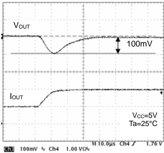
Figure 16. Transient Response (Io=1A to 2A, 10µs)
