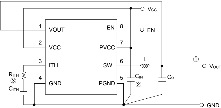
Figure 32. Layout Diagram
