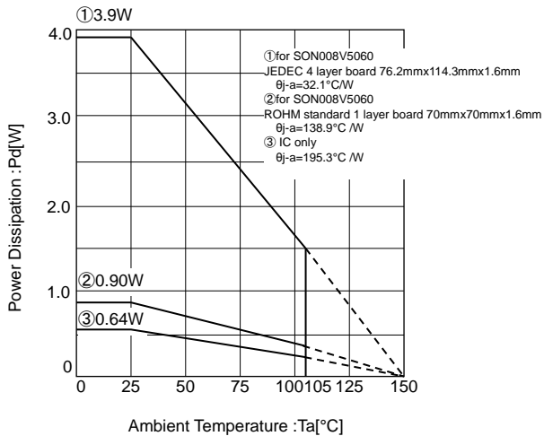
Figure 25. Thermal Derating Curve (SON008V5060)
