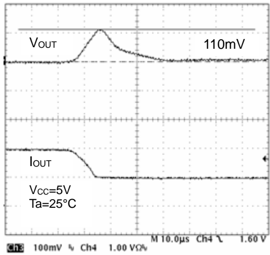
Figure 17. Transient Response (Io=2A to 1A, 10µs)
