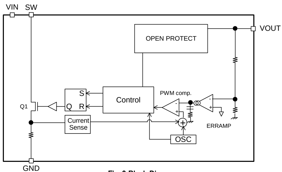
Fig. 2 Block Diagram
