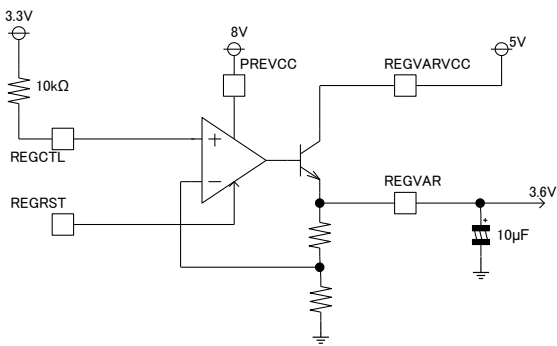
(a) Regulator 2 Controls ON/OFF of regulator 2 can be controlled by REGRST terminal.
