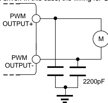
Figure 2. Snubber Circuit
