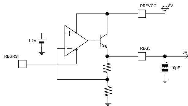
(a) Regulator 1 Control ON/OFF of regulator 1 can be controlled by REGRST terminal.
