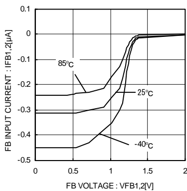
Fig.7 DC/DC Error Amp Input Bias Current
