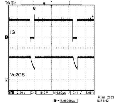
Fig.18 Gate-shading Waveform
