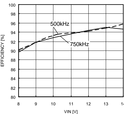
Fig.18 STEP UP EFFICIENCY
