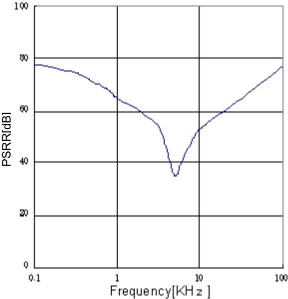
Figure 32. PSRR( I_o=0 mA)
