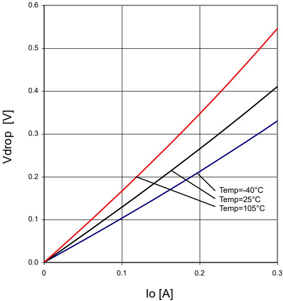
Figure 34. Minimum dropout Voltage 1 ( V_{cc}=4.5 V)
