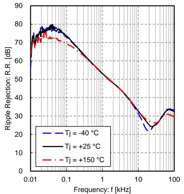
Figure 14. Ripple Rejection (V ripple = 1 V rms , I_{OUT} = 100\text{ mA} )
