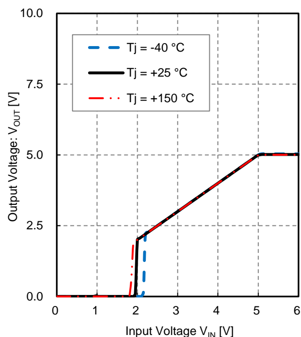
Figure 2. Output Voltage vs Input Voltage -Enlarged view
