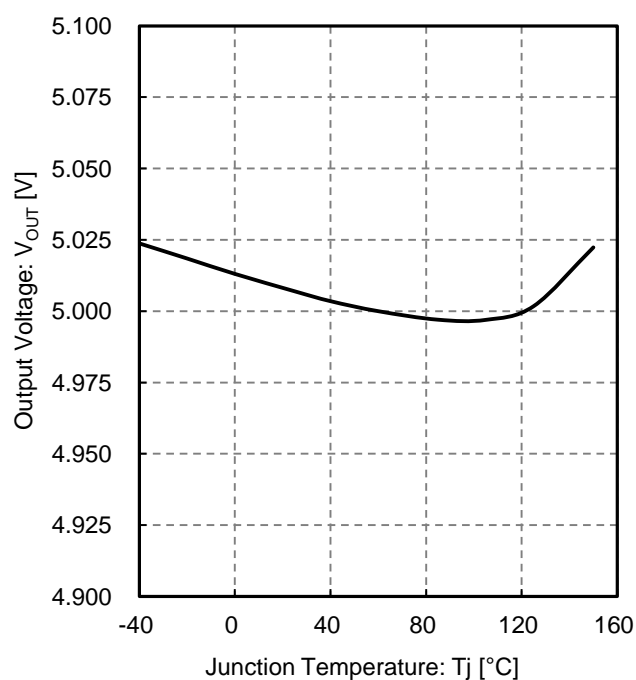
Figure 3. Output Voltage vs Junction Temperature ( I_{OUT} = 0.5 mA)
