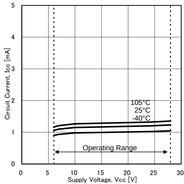
Figure 1. Circuit Current
