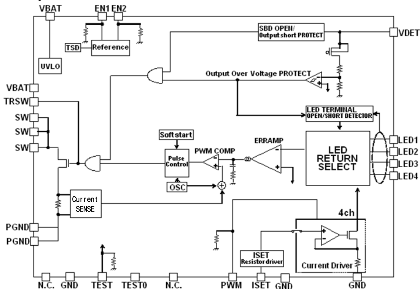
Block Diagram
