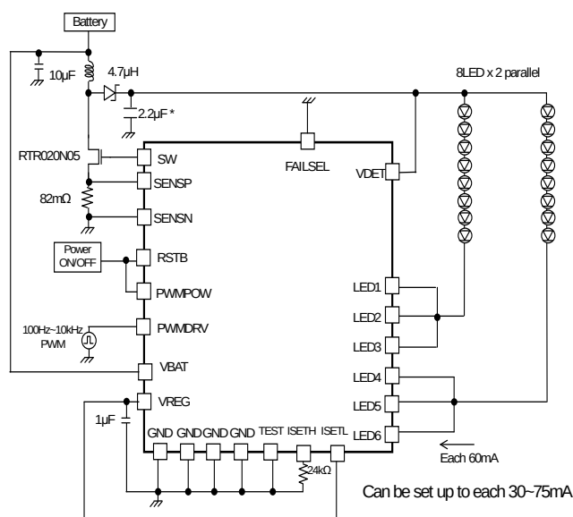
Figure 57. 8 series X 2 parallel, LED current 60mA setting Current driver PWM application
