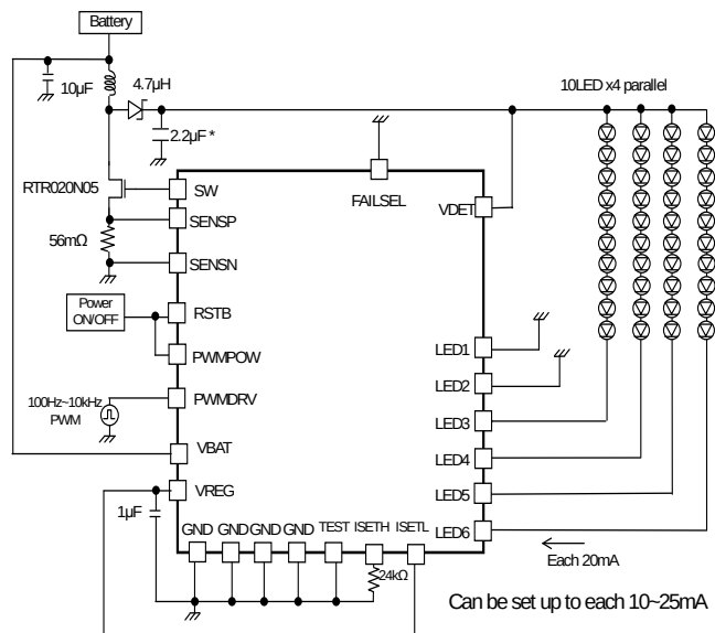
Figure 49. 10 series×4 parallel, LED current 20mA setting Current driver PWM application
