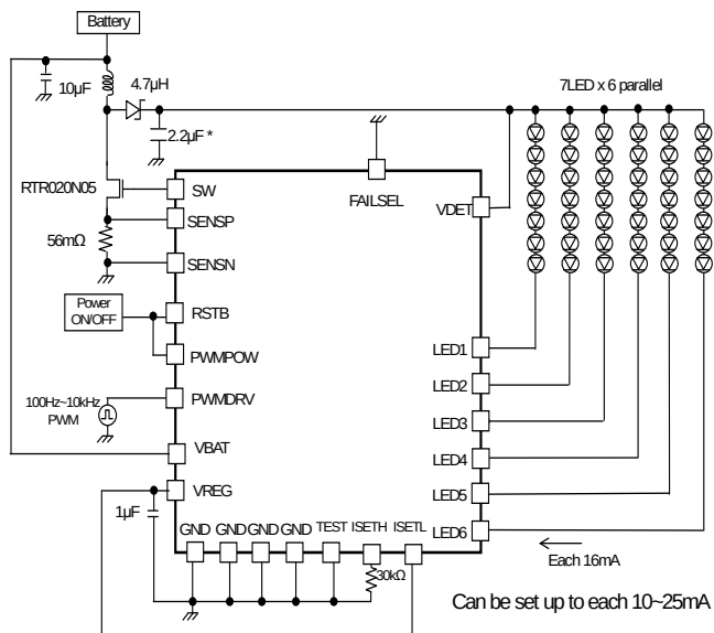
Figure 48. 7 series X6 parallel, LED current 16mA setting Current driver PWM application
