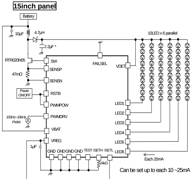
Figure 45. 10 series×6 parallel, LED current 20mA setting Current driver PWM application
