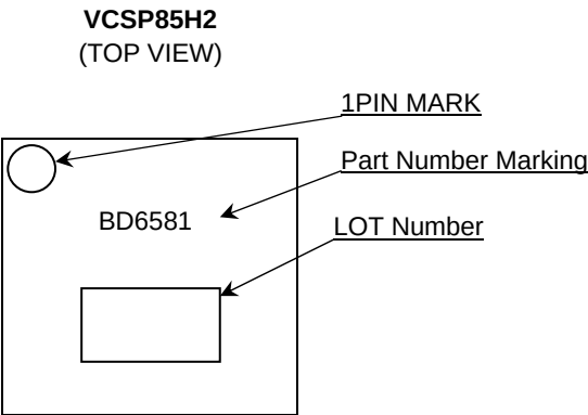
Figure 63 Marking Diagram
