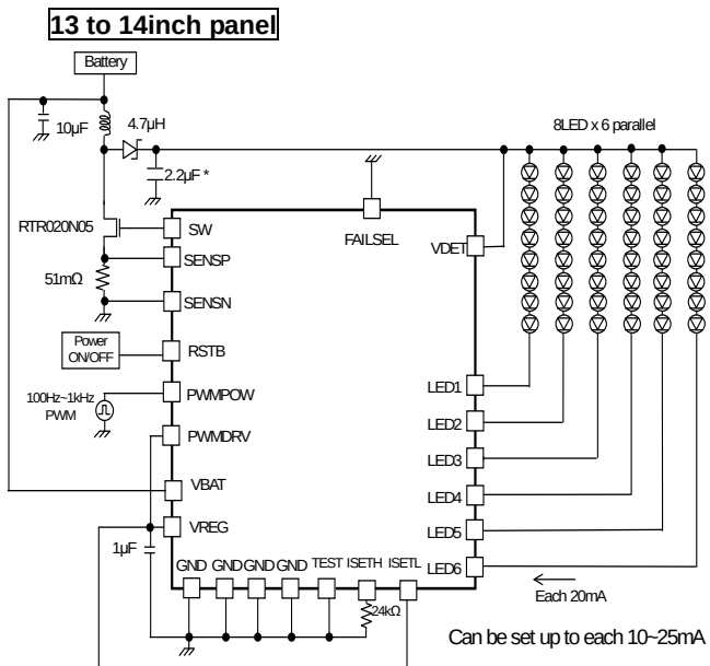
Figure 46. 8 series×6 parallel, LED current 20mA setting Power control PWM application
