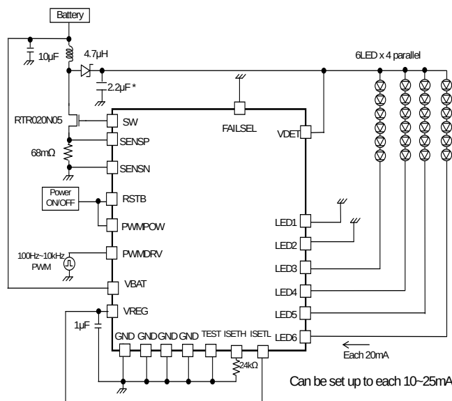
Figure 51. 6 series X4 parallel, LED current 20mA setting Current driver PWM application
