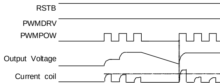
Figure 32. Light off control of PWMPOW pin at PWM control on PWM=L
