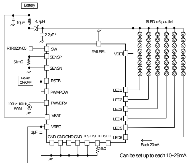
Figure 47. 8 series×6 parallel, LED current 20mA setting Current driver PWM application
