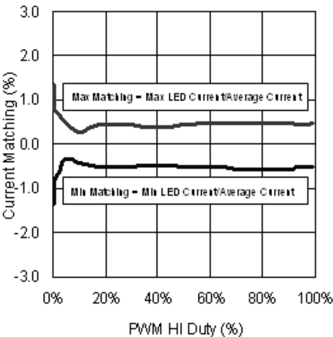
Figure 19. LED current matching vs PWM POW-HI Duty PWM = 200Hz
