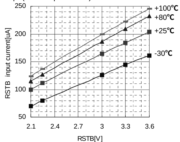
Figure 31. RSTB terminal voltage-RSTB inflow current (At the time of the current driver six lines use)
