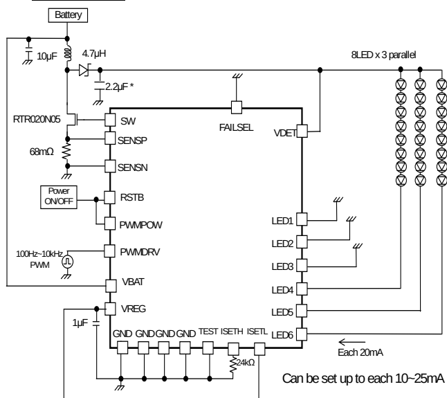
Figure 50. 8 series X3 parallel, LED current 20mA setting Current driver PWM application
