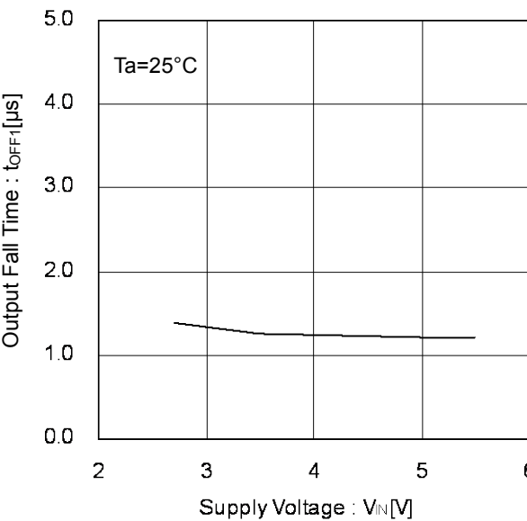
Figure 21. Output Fall Time vs Supply Voltage
