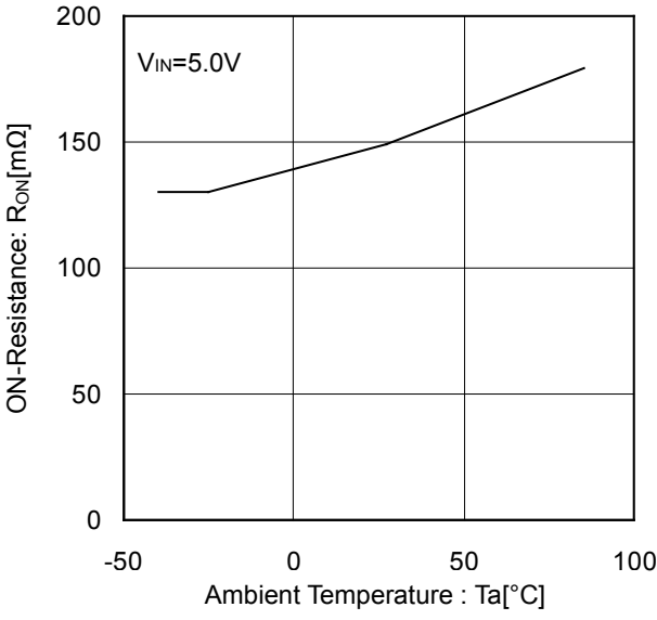
Figure 10. ON-Resistance vs Ambient Temperature
