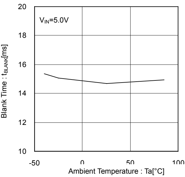
Figure 26. Blank Time vs Ambient Temperature
