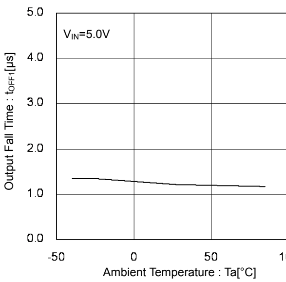
Figure 22. Output Fall Time vs Ambient Temperature
