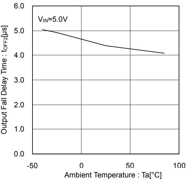
Figure 24. Output Fall Delay Time vs Ambient Temperature
