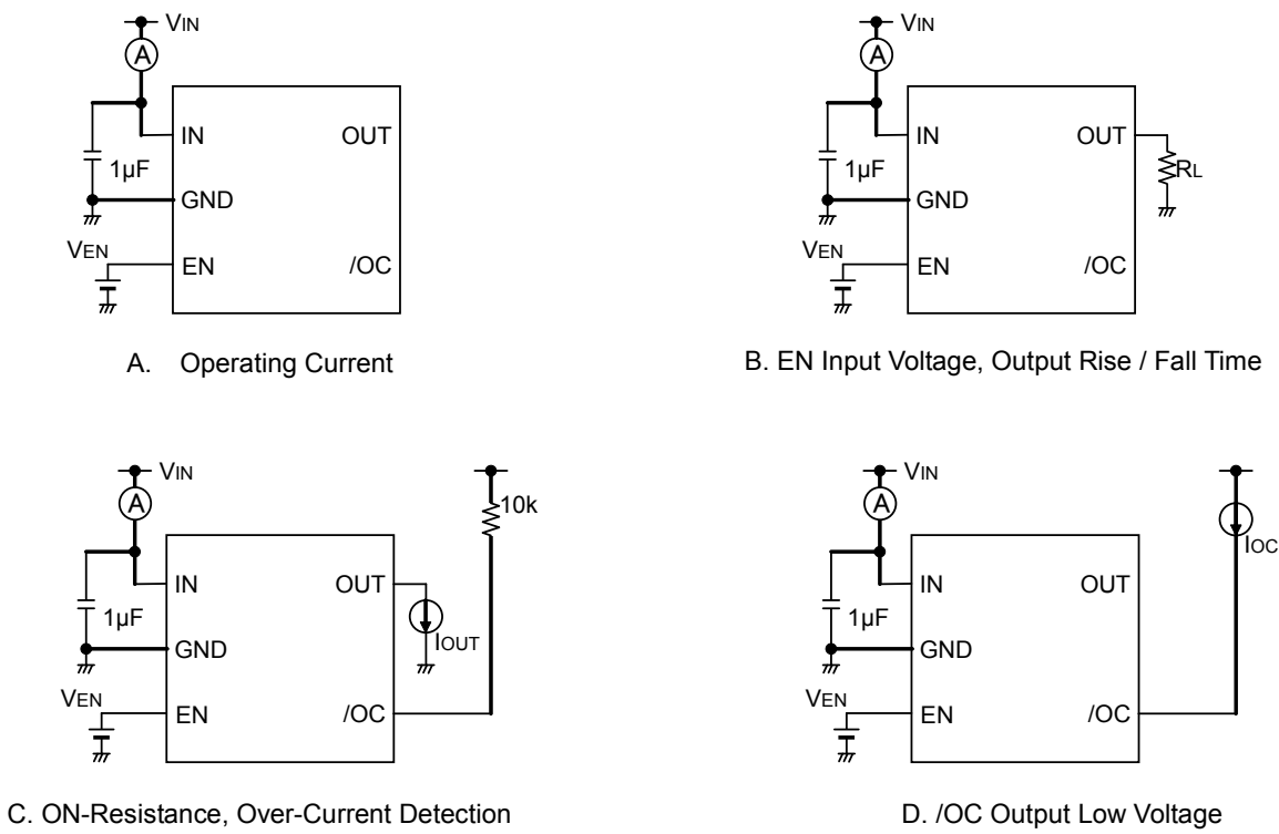
Figure 1. Measurement Circuit
