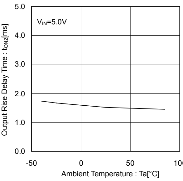
Figure 20. Output Rise Delay Time vs Ambient Temperature
