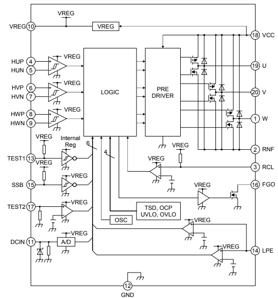
Figure 3. Block Diagram
