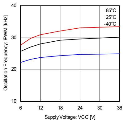
Fig.7 VCC - Carrier frequency
