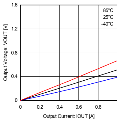
Fig.20 Output low voltage (1A class)
