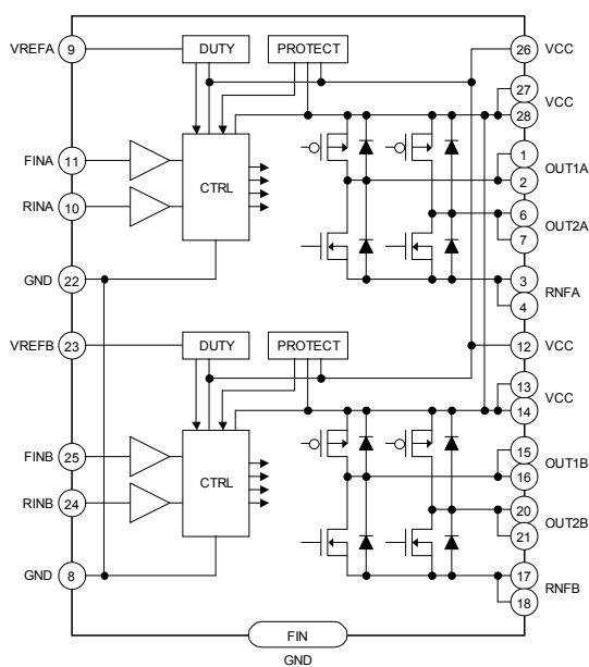
Fig.35 BD6237FM
