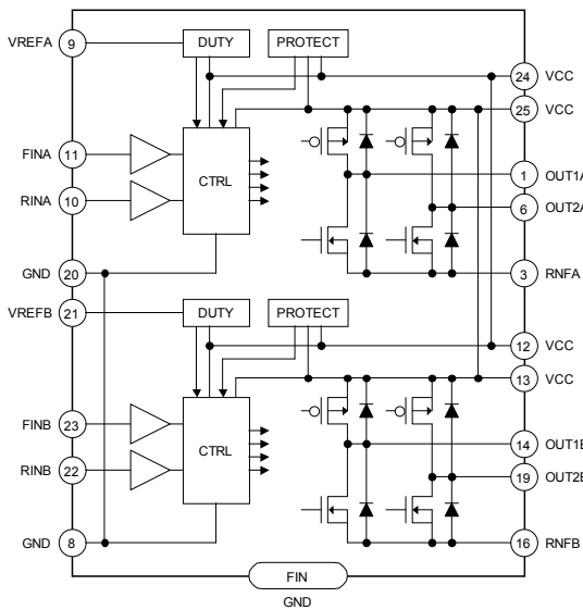
Fig.31 BD6235FP / BD6236FP
