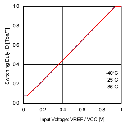
Fig.6 VREF - DUTY (VCC=24V)
