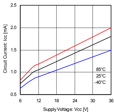
Fig.1 Supply current (1ch)
