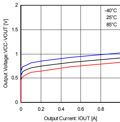
Fig.17 High side body diode (1A class)
