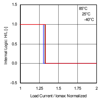
Fig.12 Over current protection (L side)
