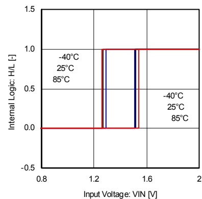
Fig.3 Input threshold voltage
