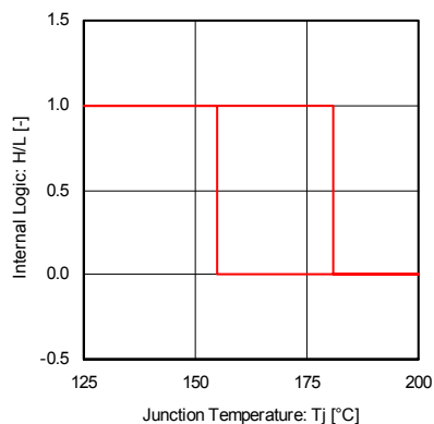
Fig.10 Thermal shutdown
