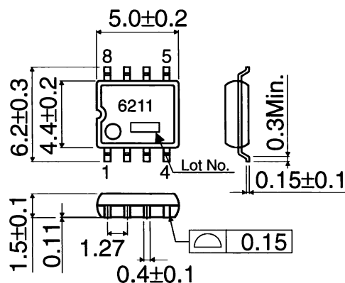
SOP8 (Unit: [mm])
