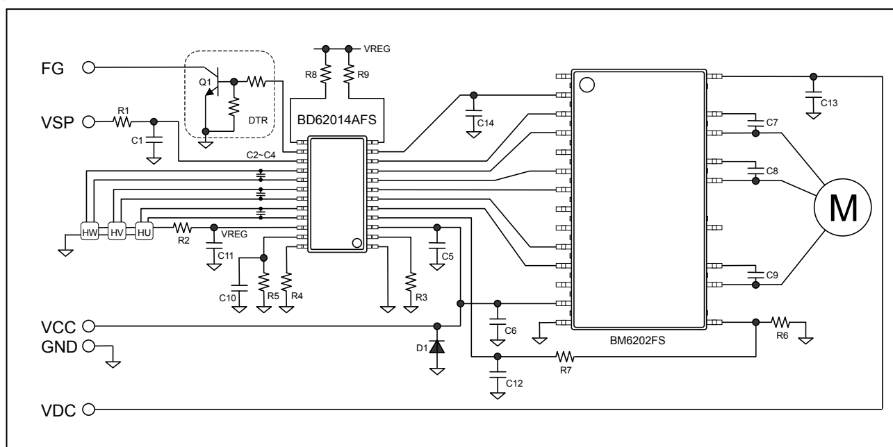
Figure 1. Application circuit example - BD62014AFS & BM6202FS
