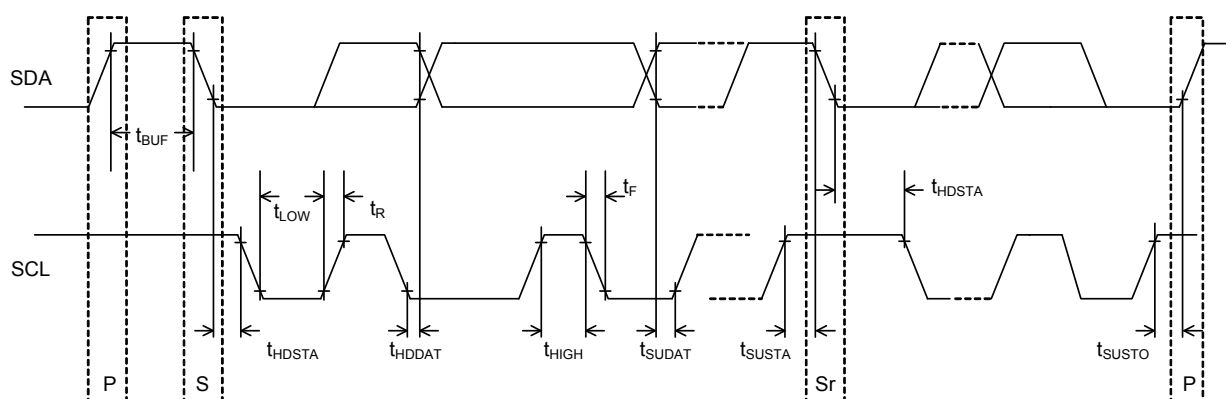
Figure 20 Timing Chart
