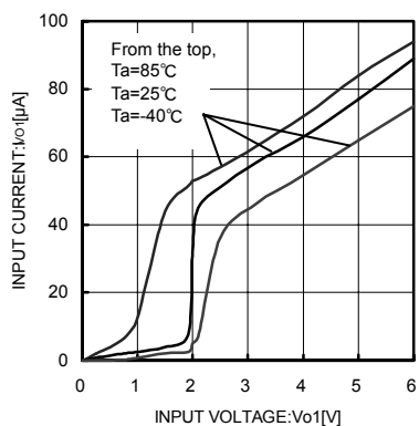
Fig.10 VO1 Sink Current
