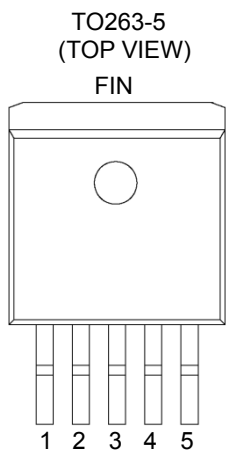
Figure 3. Pin Configuration
