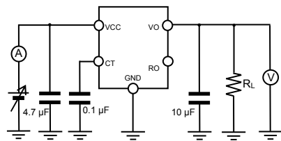
Measurement circuit for Figure. 5, 6, 7, 8, 10, 14, 15
