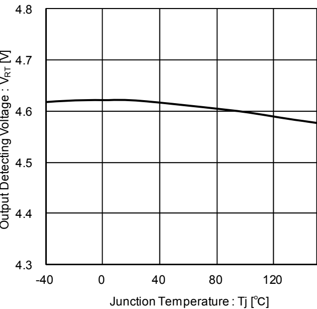
Figure 17. Output Detecting Voltage vs Temperature (R O : 10 kΩ pull-up to V O )
