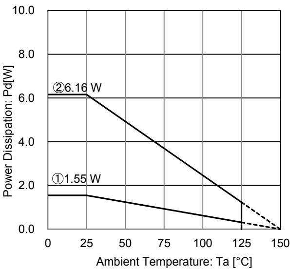
Figure 22. Package Data (TO263-5)
