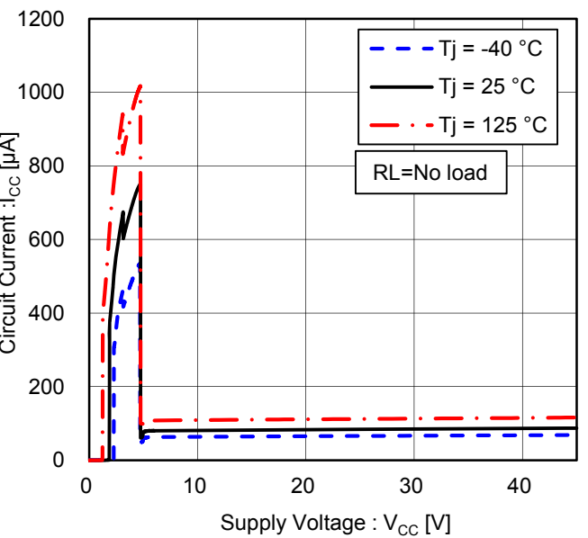
Figure 8. Circuit Current vs Supply voltage ( R_L = \text{No load} )
