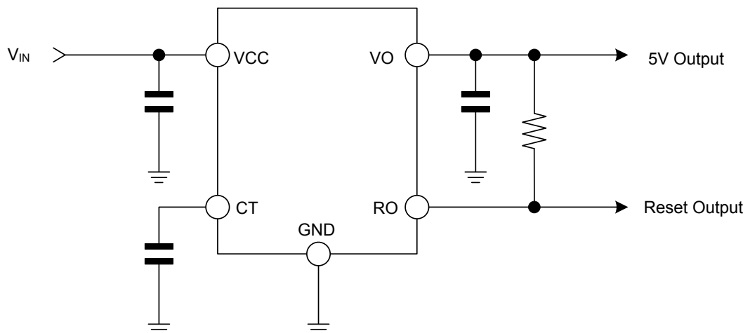
Figure 2. Application Circuit
