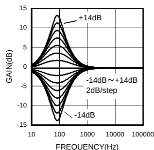
Fig.12 Bass Gain - Frequency (BD3403FV, BD3861FS)
