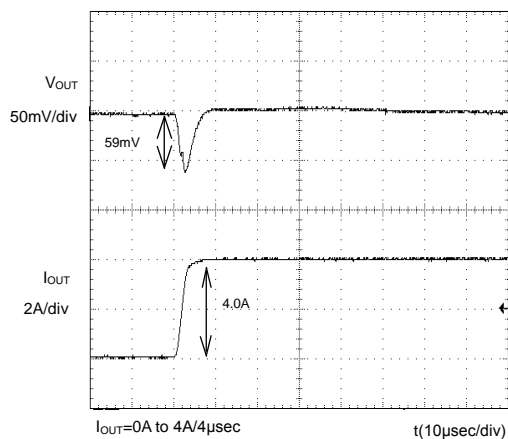
Figure 2. Transient Response (0A to 4A) C_{OUT}=100\mu\text{F}
