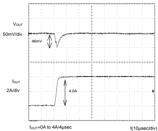
Figure 3. Transient Response (0A to 4A) C_{OUT}=100\mu\text{F} , C_{FB}=1000\text{pF}
