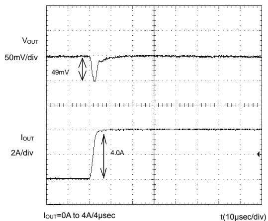
Figure 1. Transient Response (0A to 4A) C_{OUT}=22\mu\text{F} , C_{FB}=1000\text{pF}
