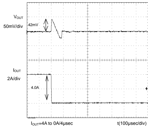
Figure 4. Transient Response (4A to 0A) C_{OUT}=22\mu\text{F} , C_{FB}=1000\text{pF}
