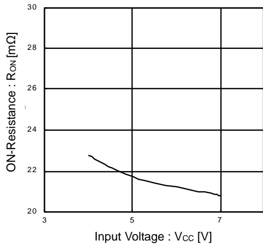
Figure 22. ON-Resistance vs Input Voltage 1 (VOUT=1.2V)
