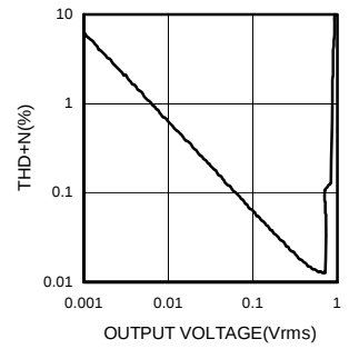
Fig.21 Total Harmonic Distortion ratio - Output Voltage (REC)
