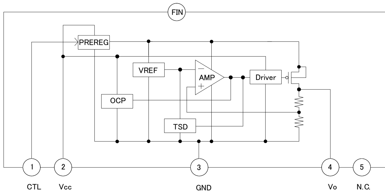
Figure 5. Block diagram BDxxFD0WHFP/FP2 (Output Voltage Fixation Type)
