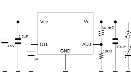
Measurement setup for Figure 11,12.
