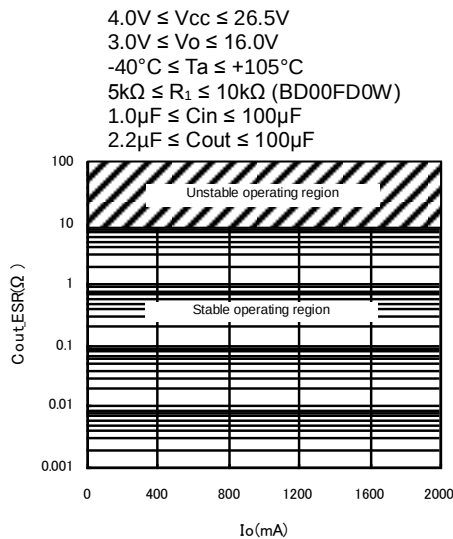
C_{out} ESR vs I_o 3.0\text{V} \leq V_o \leq 16.0\text{V}
