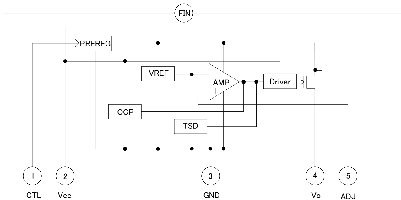
Figure 4. Block diagram BD00FD0WHFP/FP2 (Output Voltage Variable Type)
