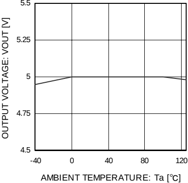
Fig. 11 Output Voltage vs Temperature
