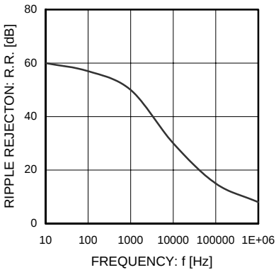
Fig. 5 Ripple Rejection
