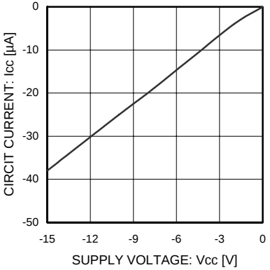
Fig. 9 Back Current
