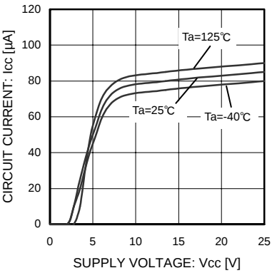
Fig. 1 Circuit Current
