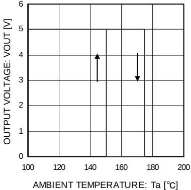
Fig. 12 Thermal Shutdown Circuit
