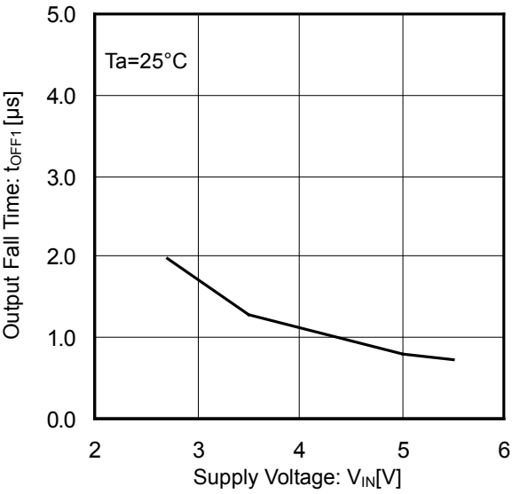
Figure 22. Output Fall Time vs Supply Voltage
