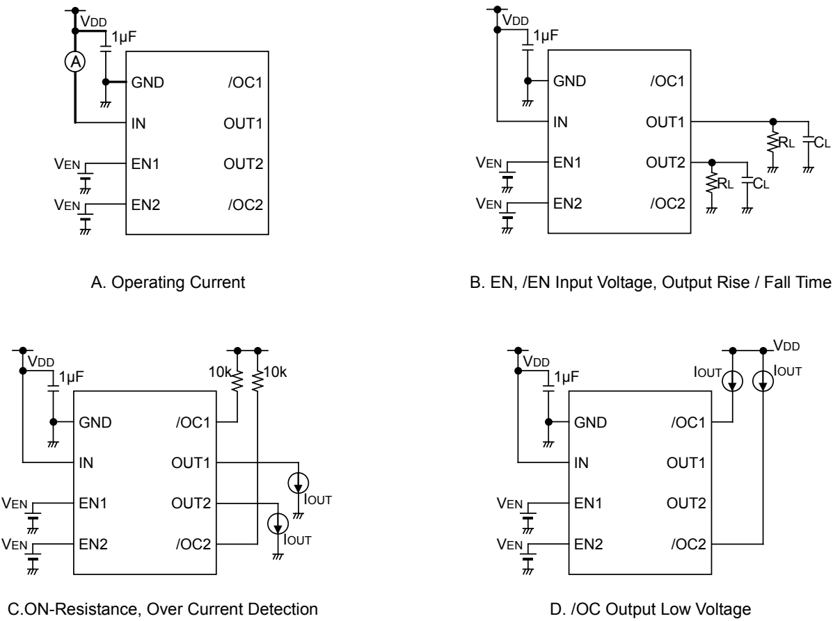
Figure 1. Measurement Circuit
