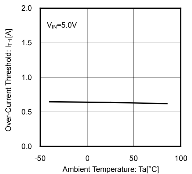
Figure 15. Over-Current Threshold vs Ambient Temperature
