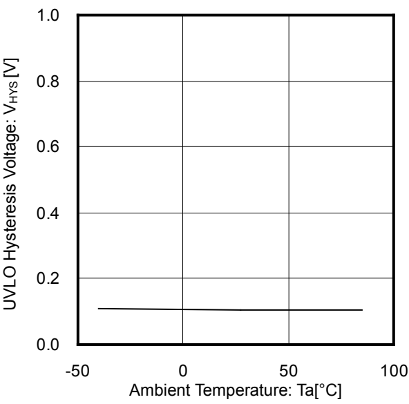
Figure 29. UVLO Hysteresis Voltage vs Ambient Temperature
