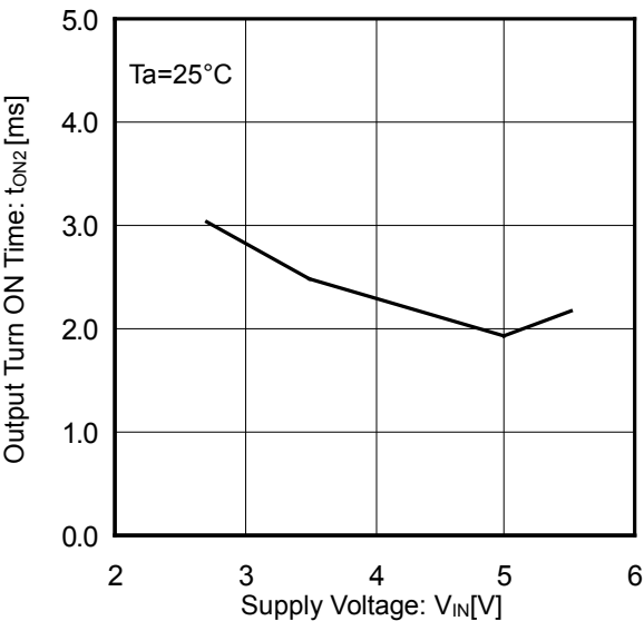
Figure 20. Output Turn ON Time vs Supply Voltage
