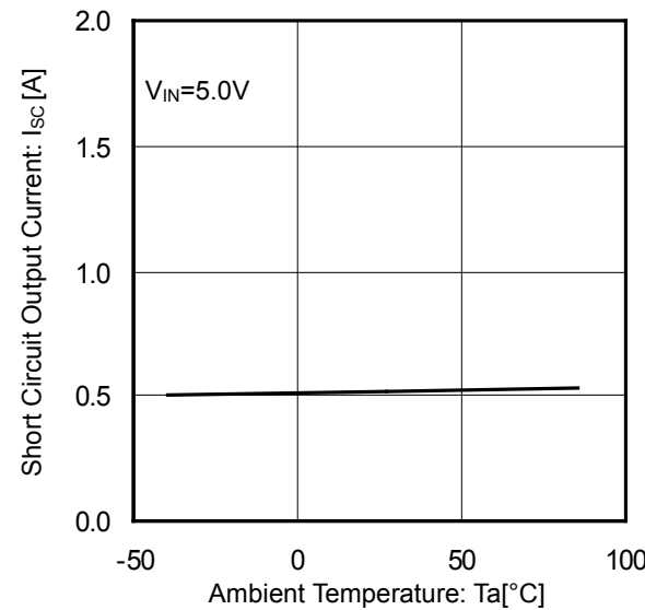
Figure 17. Short Circuit Output Current vs Ambient Temperature
