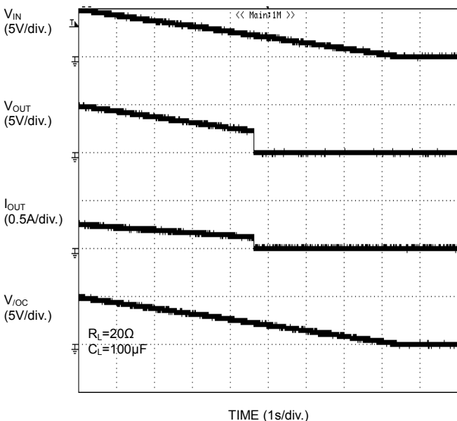
Figure 39. UVLO Response when Decreasing V_{IN} (BD2056AFJ)
