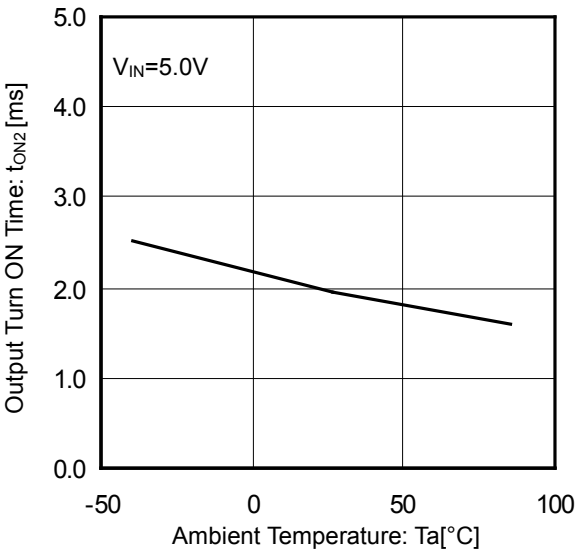
Figure 21. Output Turn ON Time vs Ambient Temperature
