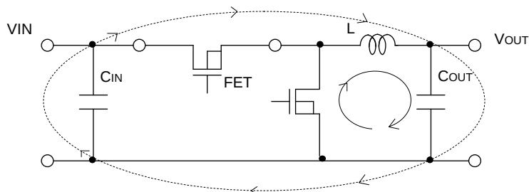
Fig.26 Current loop in Buck regulator system
