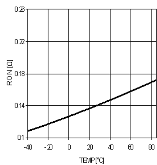
Fig.8 Hi,Low-Side On-resistance
