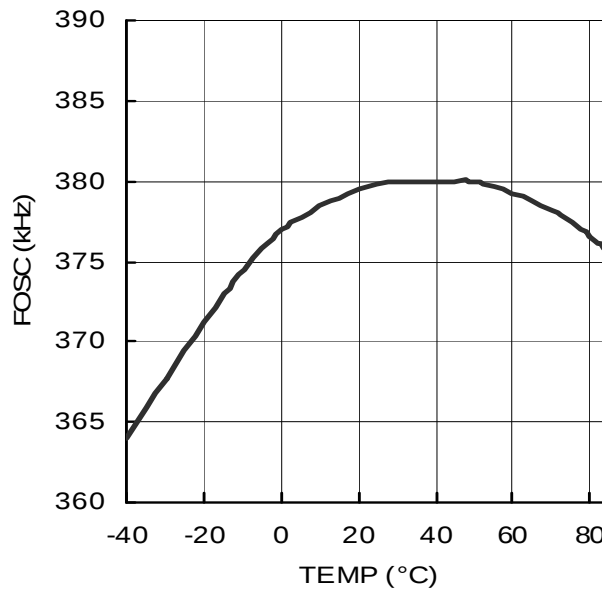
Fig.9 Operating Frequency
