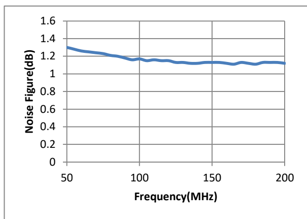
Figure 8. Noise Figure(NF)
