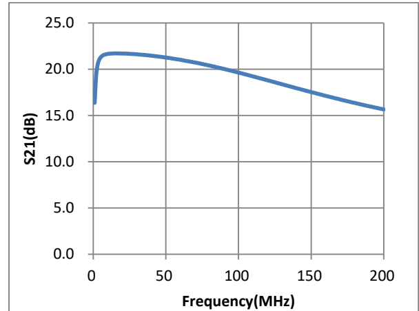
Figure4. Power Gain(S21)
