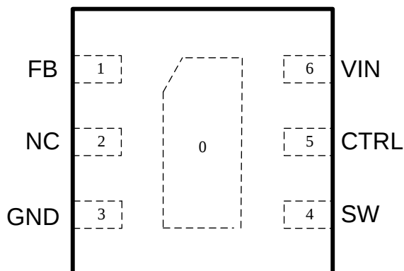
DFN2x2-6L
