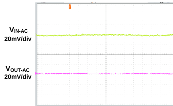
Output Ripple
