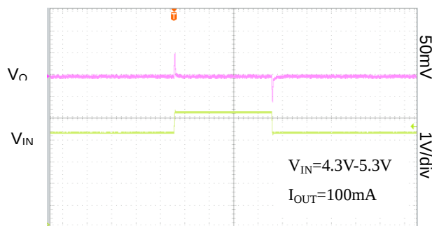
Line Transient Response
