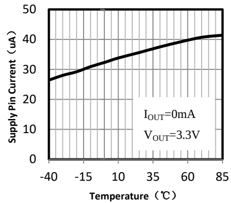
Supply Pin Current vs. Temperature
