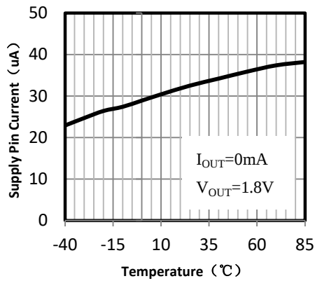
Supply Pin Current vs. Temperature
