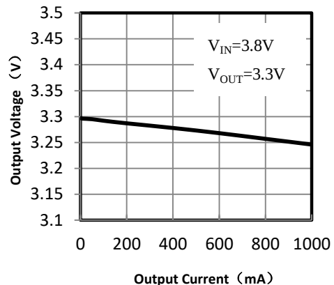
Load Regulation
