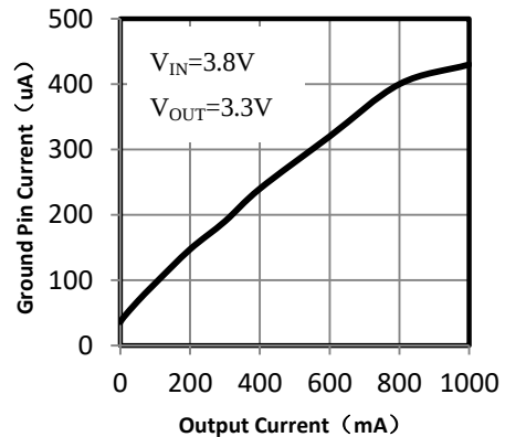
Ground Pin Current vs. Output Current
