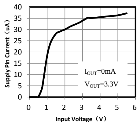
Supply Pin Current vs. Input Voltage
