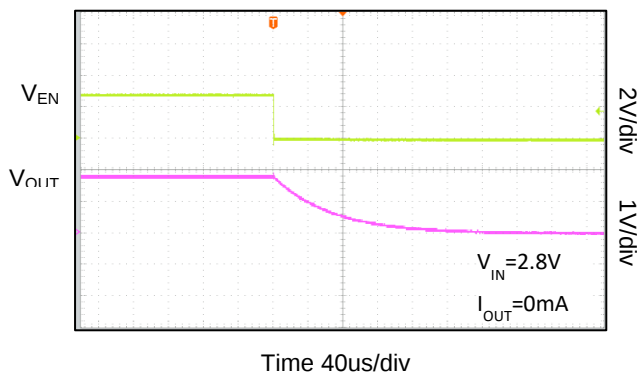
Shutdown from EN ( V_{OUT}=1.8V )
