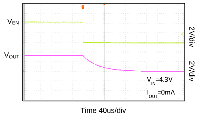
Shutdown from EN ( V_{OUT}=3.3V )
