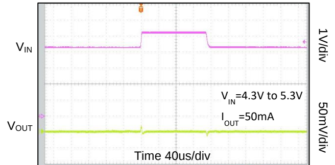
Line Transient Response ( V_{OUT}=3.3V )
