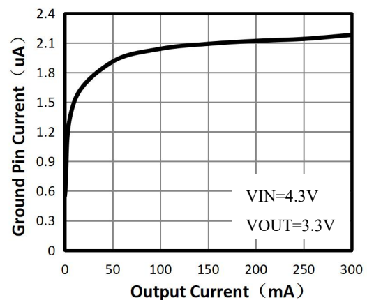
Ground Pin Current vs. Output Current
