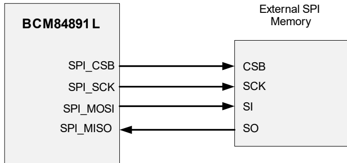
Figure 13: SPI Serial Interface Block Diagram
