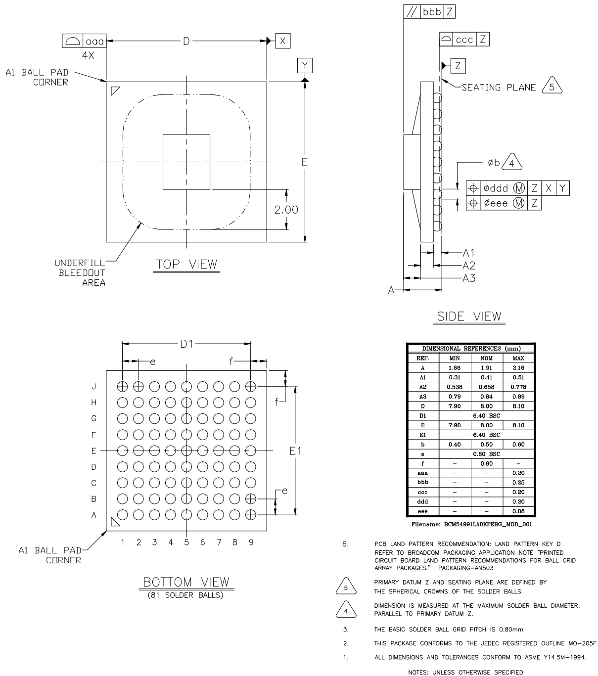
Figure 26: BCM84891LA0KFBSBG/BCM84891LA0IFBSBG Outline Drawing (8 mm × 8 mm Package)
