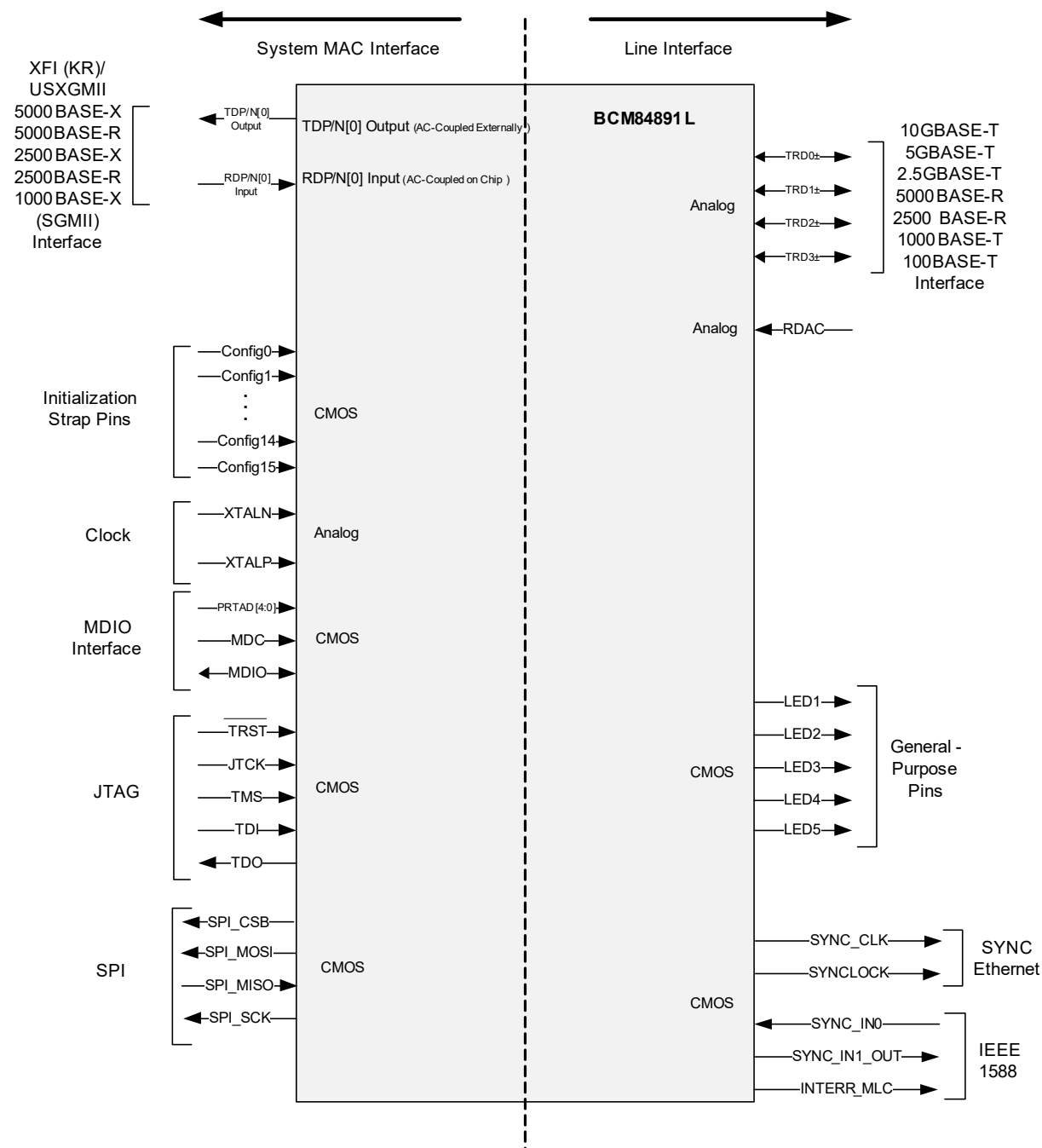
Figure 2: Interface Block Diagram Per-Port
