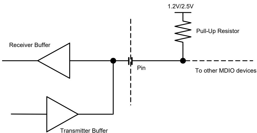
Figure 11: MDIO Interface
