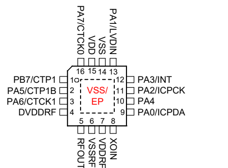
BC68F3132 16 QFN-A
