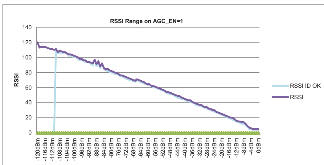
RSSI Reading Curve when AGC Enabled
