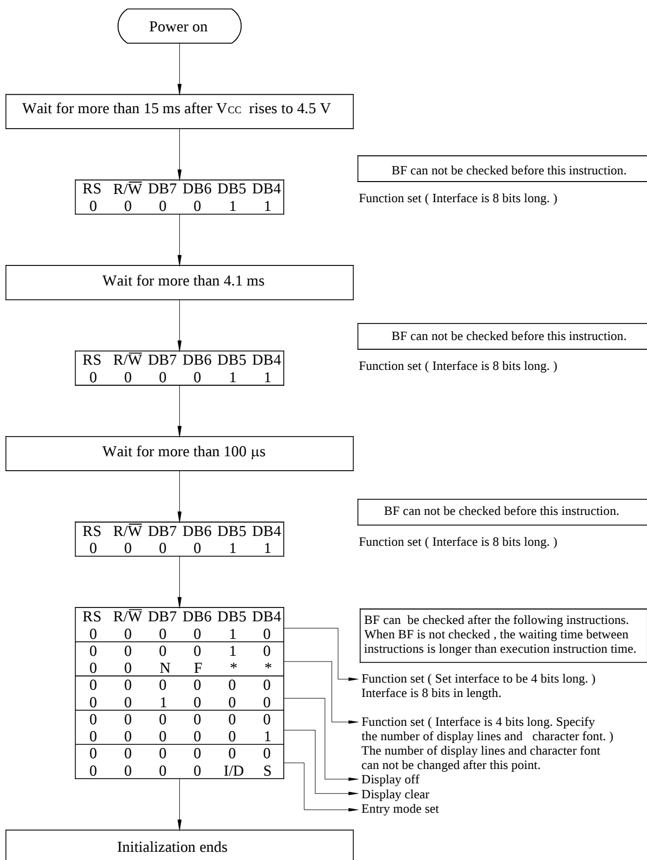
4-Bit Ineterface
