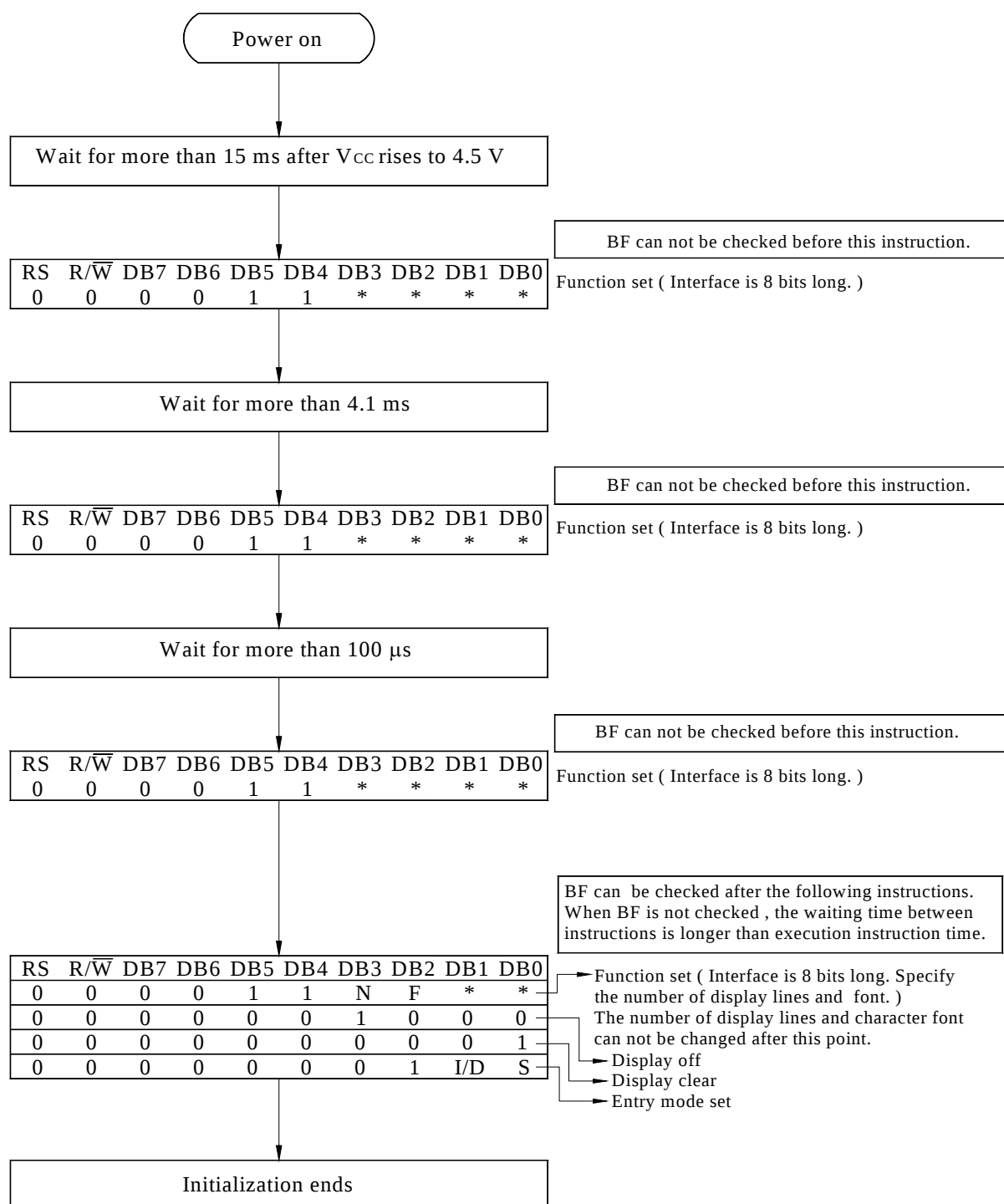
8-Bit Ineterface
