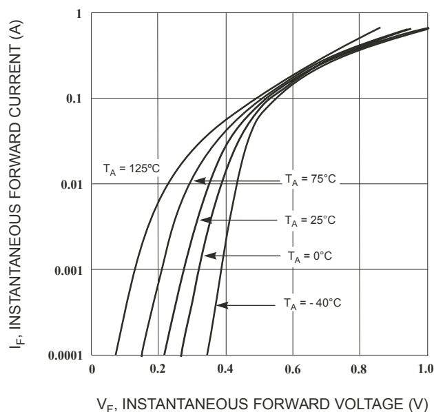
Fig. 2 Forward Characteristics
