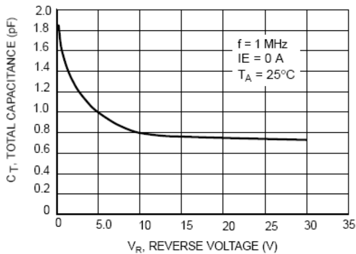
Figure 4. Total Capacitance
