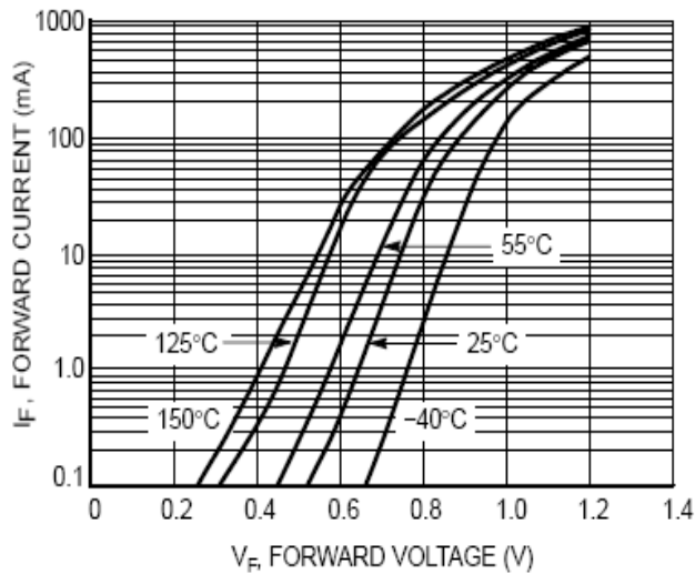
Figure 2. Forward Current
