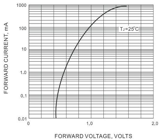
FIG. 1-TYPICAL FORWARD CHARACTERISTIC
