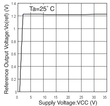
Fig. 8 Reference output voltage vs. Power supply voltage (BA9744FV)
