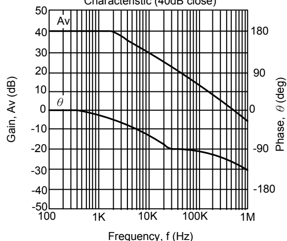
Figure 5. Error Amplifier AC Gain Characteristic (40dB close)
