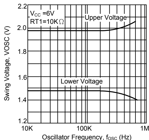
Figure 3. Swing Voltage vs. Frequency
