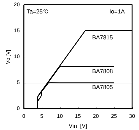
Fig.15 Line Regulation ( I_o=1\text{A} )
