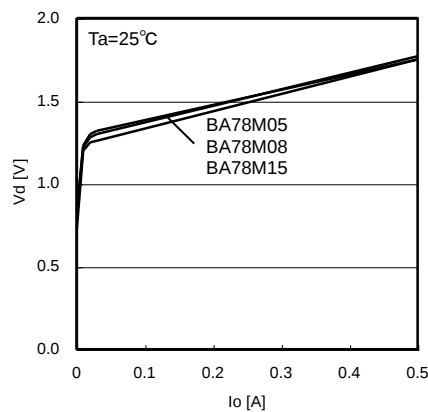
Fig.7 Dropout Voltage
