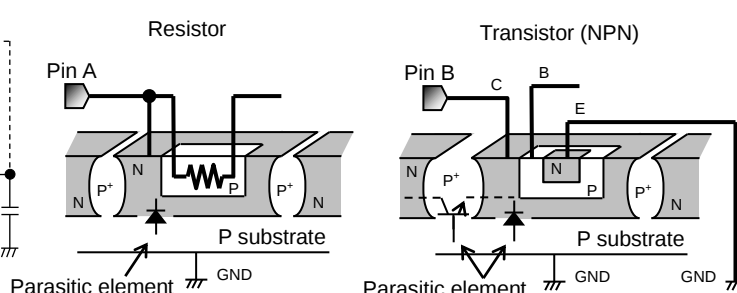
Fig.28 Simplified structure of monoristic IC
