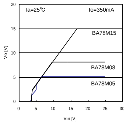
Fig.2 Line Regulation ( I_o=350\text{mA} )
