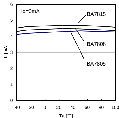
Fig.23 T_a - I_b
