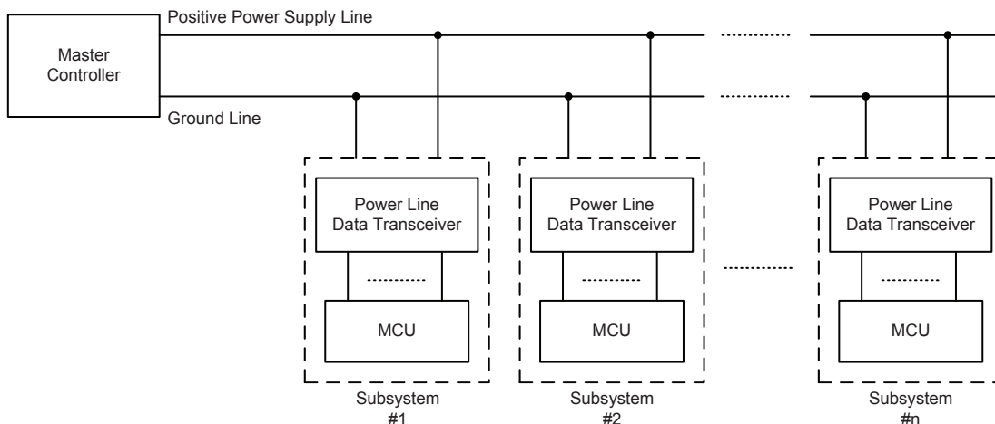
Power Line Data Transceiver System Block Diagram
