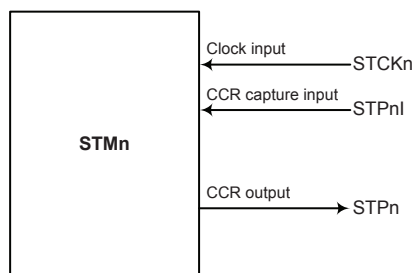
STM Function Pin Control Block Diagram (n=0~1)
