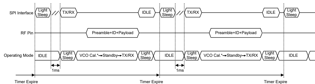
Periodical TX/RX Timing
