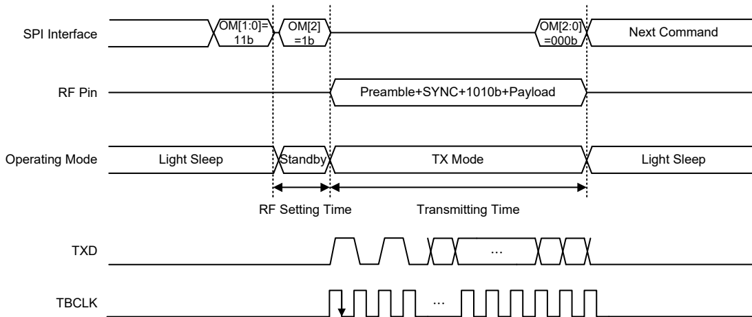
TX Timing in Direct Mode
